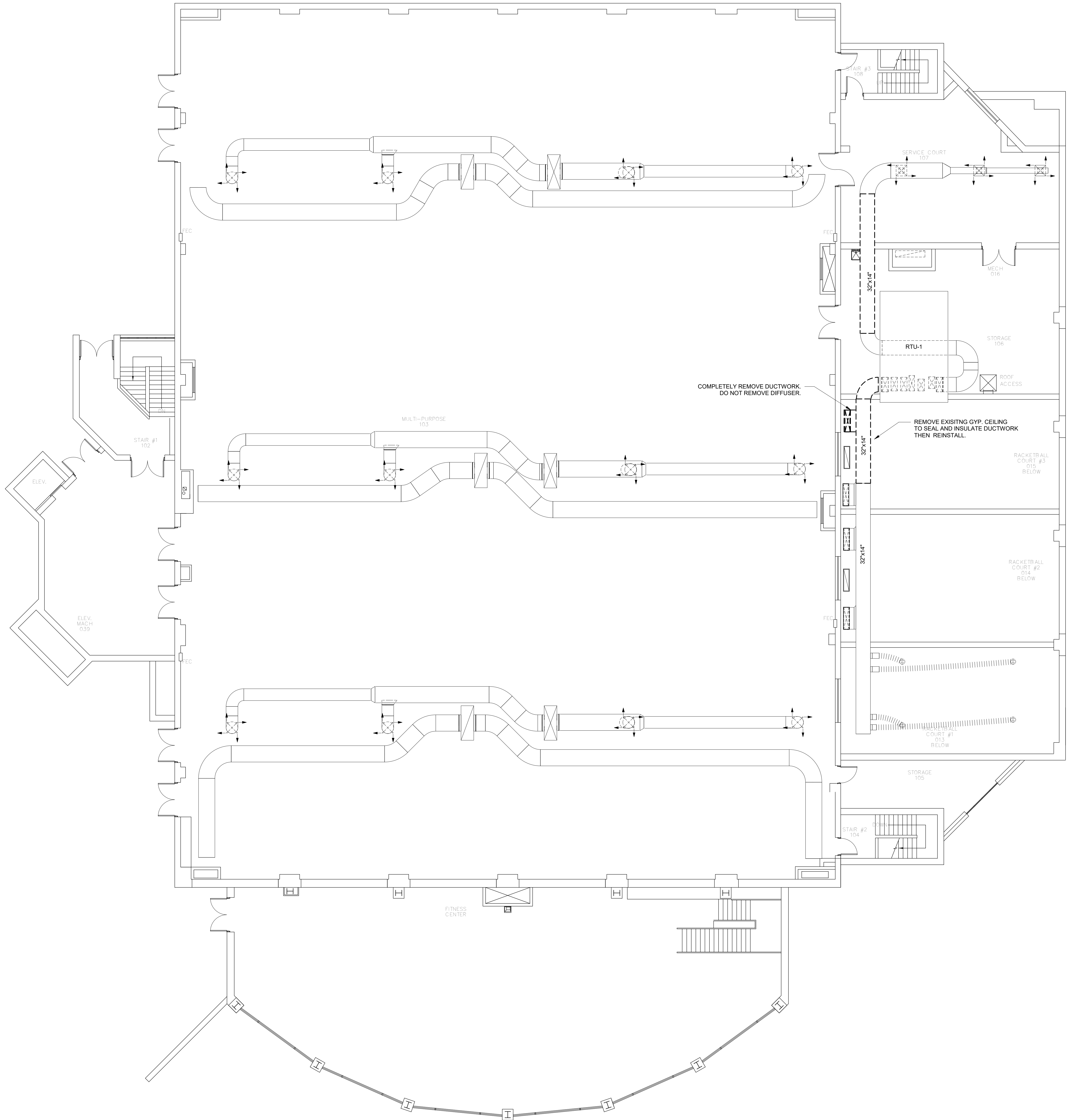
1 MECHANICAL DEMOLITION - UPPER LEVEL SCALE: 1/8" = 1'-0"
